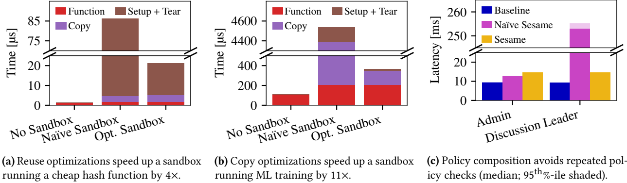
Figure 10. Drill-down experiments: Sesame benefits from sandbox reuse reducing setup/teardown overhead (a) and from direct copies avoiding serialization of data passed into the sandbox (b); policy composition reduces check overheads (c). Functions run 2× slower in the sandbox because of the WASI runtime [11] and inserted dynamic checks, e.g., on pointer dereferencing.
